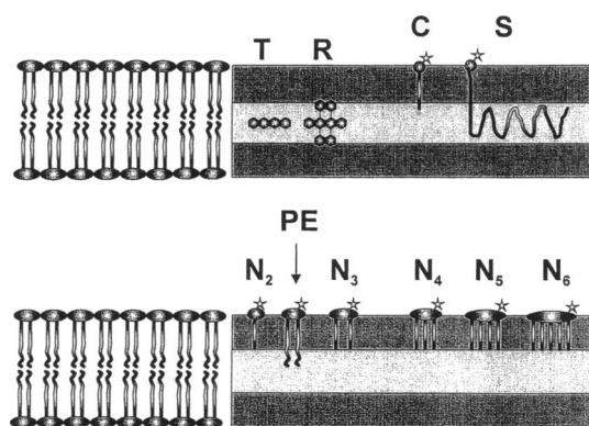
FIGURE 4 Diagrammatic representation of the "triple layer" model for a membrane. The darker region represents the \sim 1-nm-thick viscous region close to the surface, and the lighter region represents the 1–1.5-nm-thick fluid region in the hydrophobic interior. A series of molecules are depicted: T, tetracene; R, rubrene; C, NBD-labeled citronellol; S, NBD-labeled solanosol; PE, NBD-labeled phospholipid analog; N n , NBD-labeled macrocycle with n nitrogens in the ring (see text). The diffusion data suggest that C, S, PE, N 2 (N 2 L[NBD]), and N 3 (N 3 L 2 [NBD]) have the same diffusion coefficient because they are comparable in size to the lipid molecule, and the bulk in the interior is of no consequence. The diffusion rates of N 4 (N 4 L 3 [NBD]), N 5 (N 5 L 4 [NBD]), and N 6 (N 6 L 5 [NBD]) are slower because their size in the viscous region of the membrane is larger than that of the host lipid.
